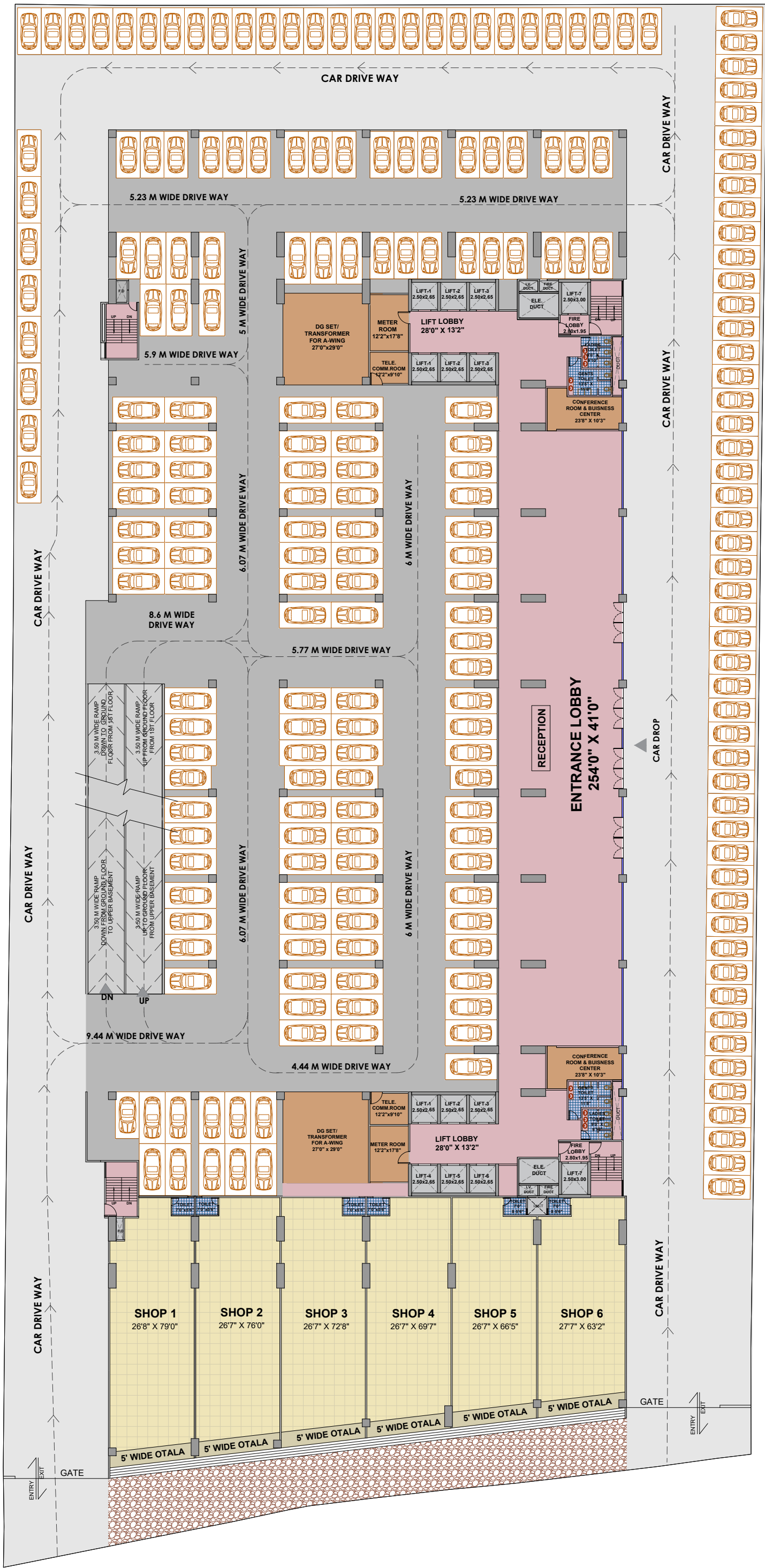
GROUND FLOOR + STILT PARKING PLAN
